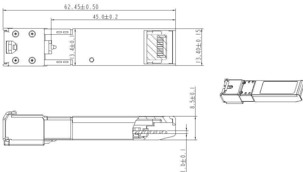
Figure 3-1 OM5070AX100 mechanical dimensions
