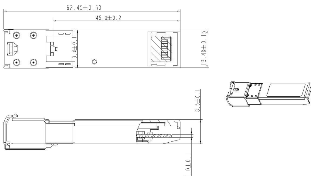
Figure 3-1 OM5071AX100 mechanical dimensions
