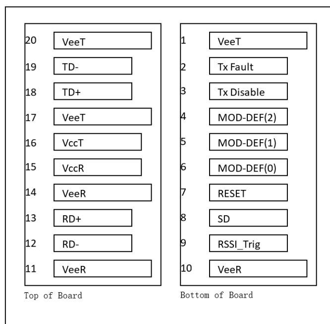
Figure 2-1 MSA compliant connector
