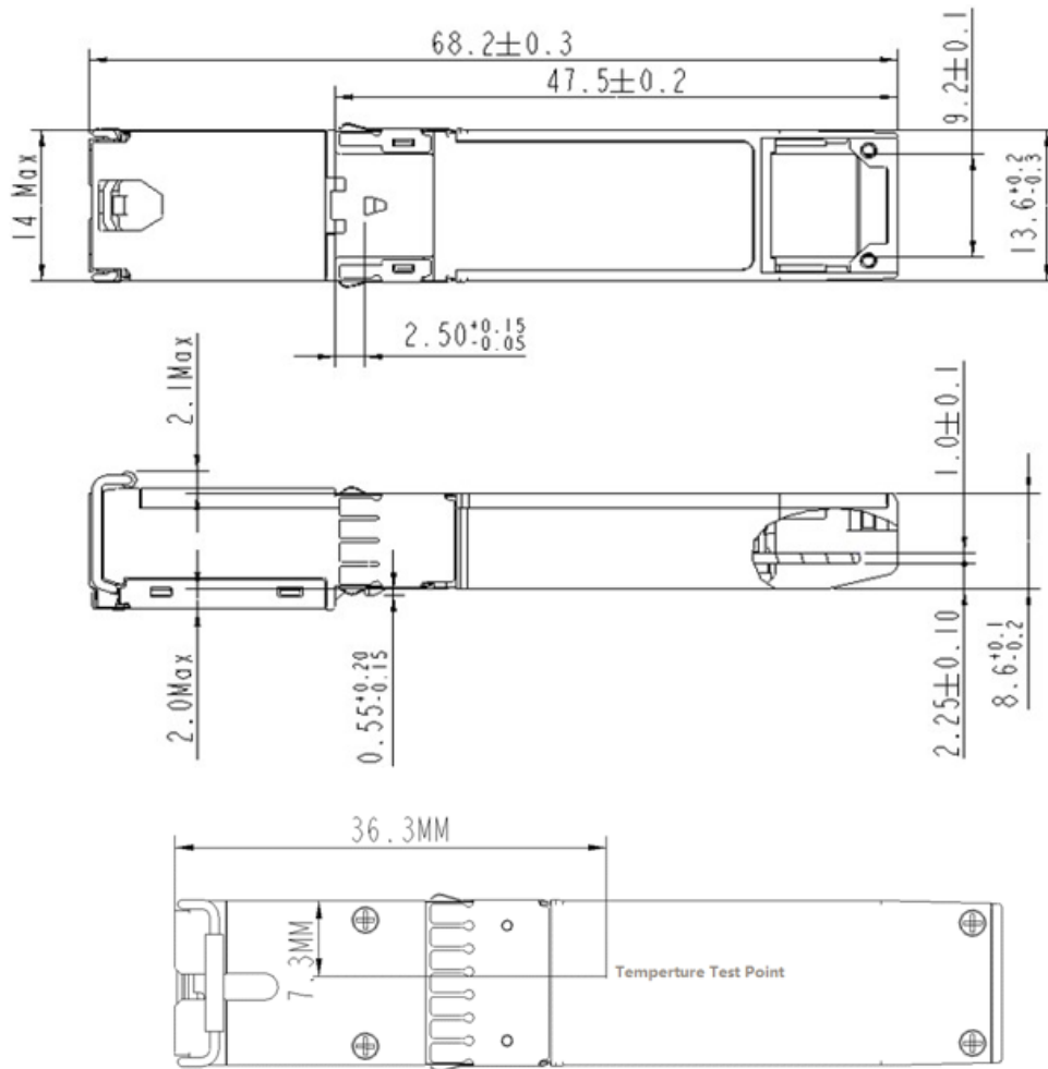
Figure 3-1 OM5270SX500 mechanical dimensions
